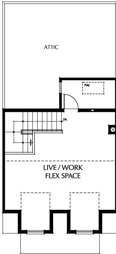
THIRD FLOOR
